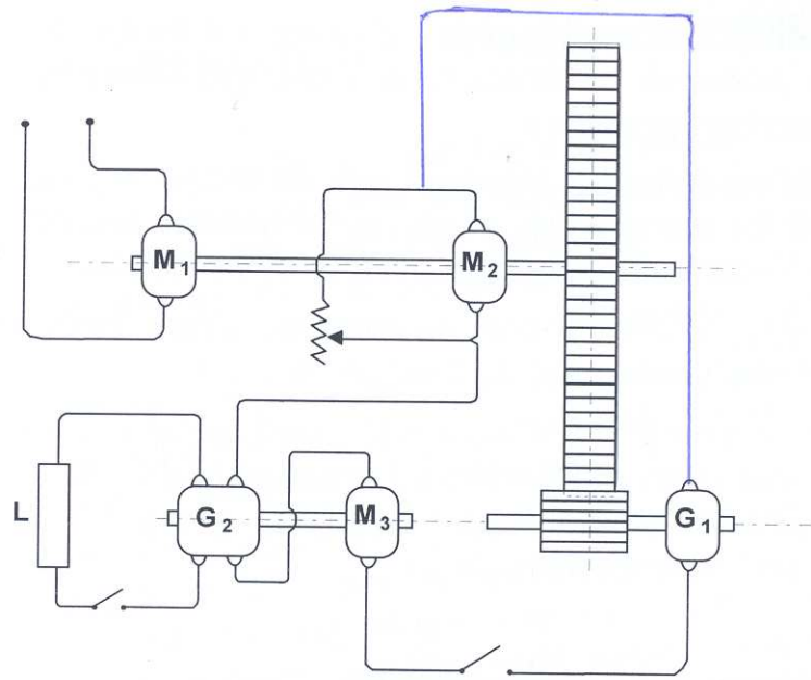
Fig. 20: The general layout of Bandiko's Perpetual Motion Machine. M_1 is the motor used to start the machine. M_2 is the motor driving the generator G_1 . M_3 is the motor driving the generator G_2 for producing power for use. G_1 is the generator that generates the e.m.f. for driving the current through M_3 , G_2 and M_2 . G_2 is the generator that generates electricity for use.
